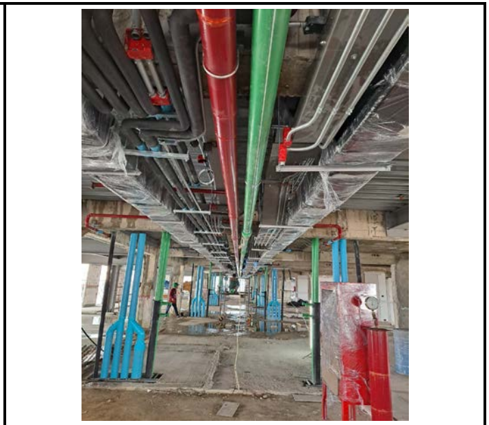
Activity Installation CW,HW Pipe Floor 16 Date : 7 September 2563
