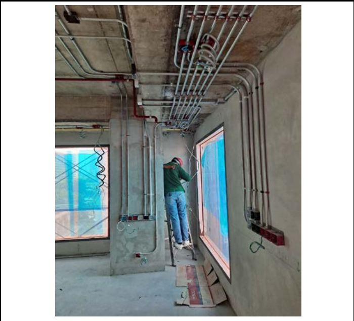
Activity Electrical System Test Mock up Room No.24 Floor 08 Date : 7 September 2563
