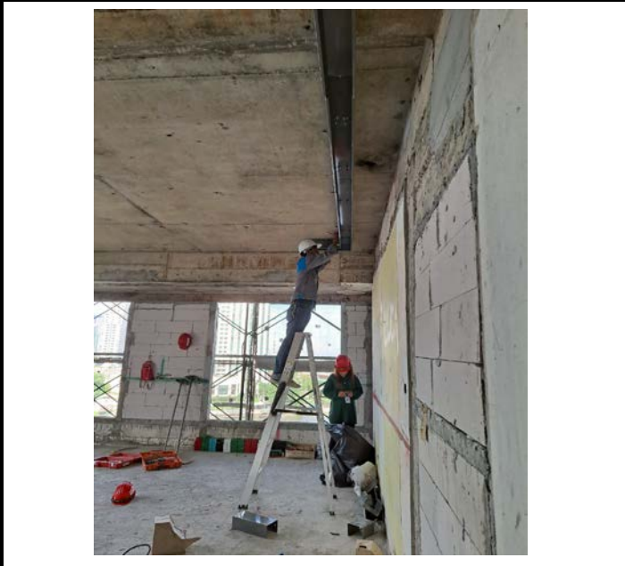
Activity Installation of Electrical Pipe Above the ceiling for the Room. Floor 13 Date : 8 September 2563
