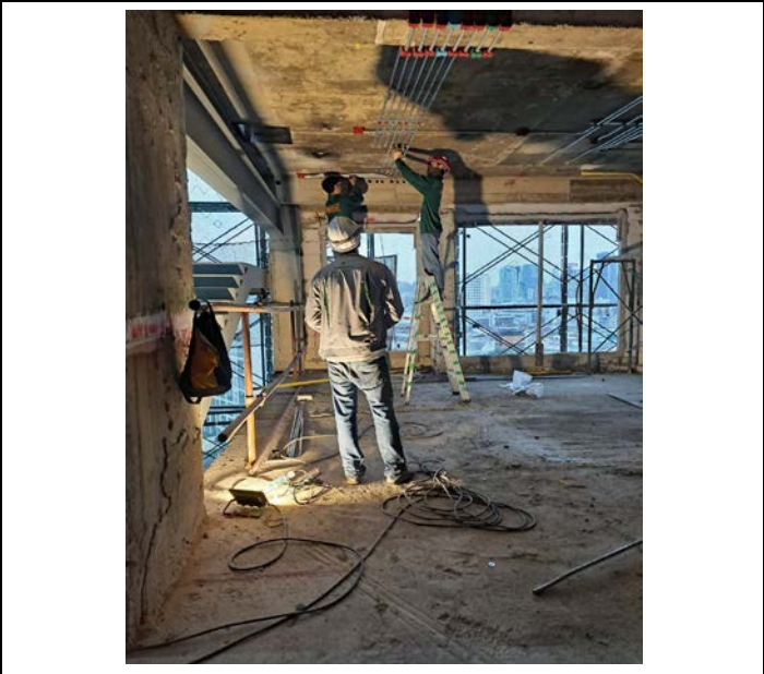
Activity Installation of Electrical Pipe Above the ceiling for the Room. Floor 14 Date : 10 September 2563
