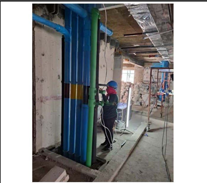
Activity Installation the Pipe Holder Floor 6-16 Date : 11 September 2563
