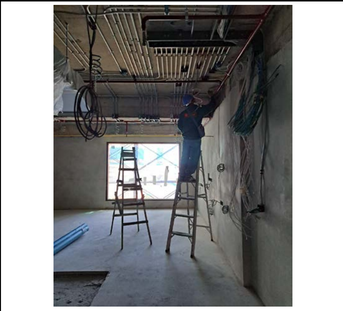
Activity Installation Air Conditioned Sewer for Mocku p Room No.24 Floor 08 Date : 11 September 2563
