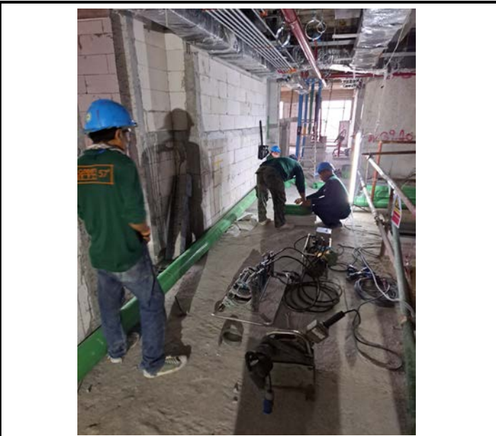
Activity Installation CW,HW Pipe Area Corridor. Floor 12 Date : 12 September 2563
