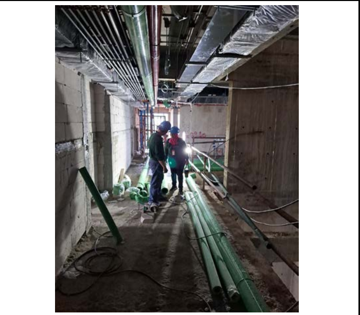
Activity Installation CW,HW Pipe Area Corridor. Floor 12 Date : 15 September 2563
