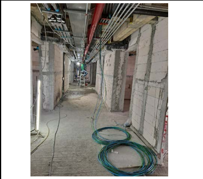
Activity Wiring the Electrical System for Corridor Floor 08 Date : 15 September 2563
