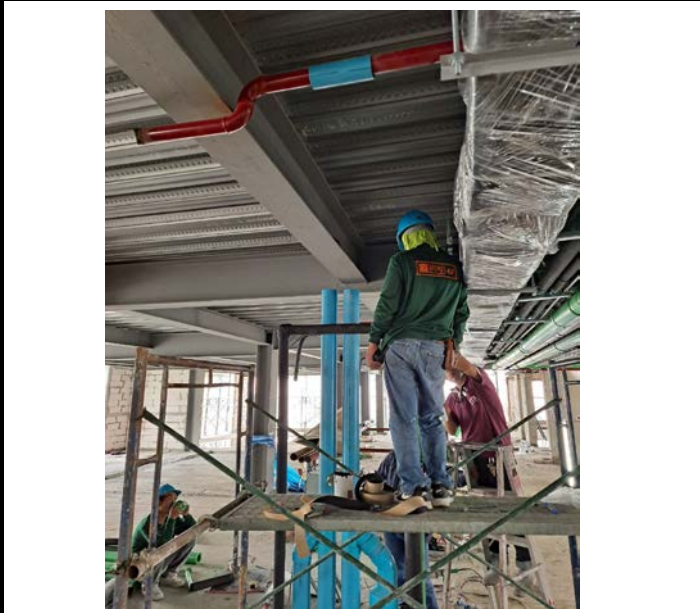
Activity Installation CW,HW Pipe Area Corridor. Floor 16 Date : 15 September 2563
