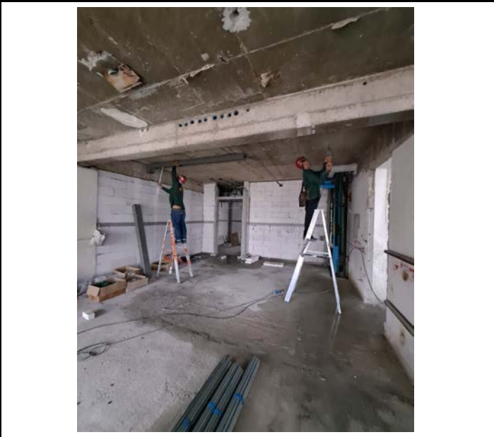
Activity Installation of Electrical Pipe Above the ceiling for the Room. Floor 13 Date : 15 September 2563
