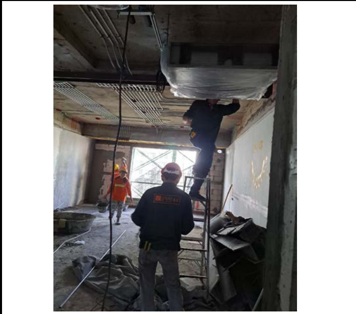
Activity Installation of Electrical Pipe Above the ceiling for the Room. Floor 08 Date : 16 September 2563
