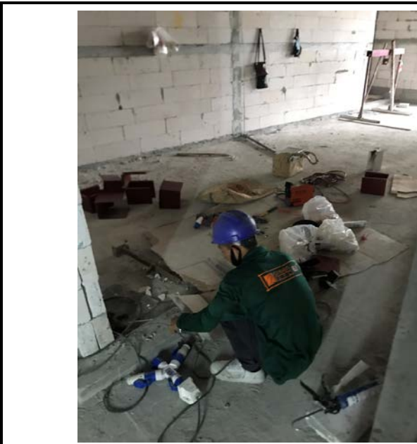
Activity Installation of Duct In The Room Floor 10 Date : 18 September 2563
