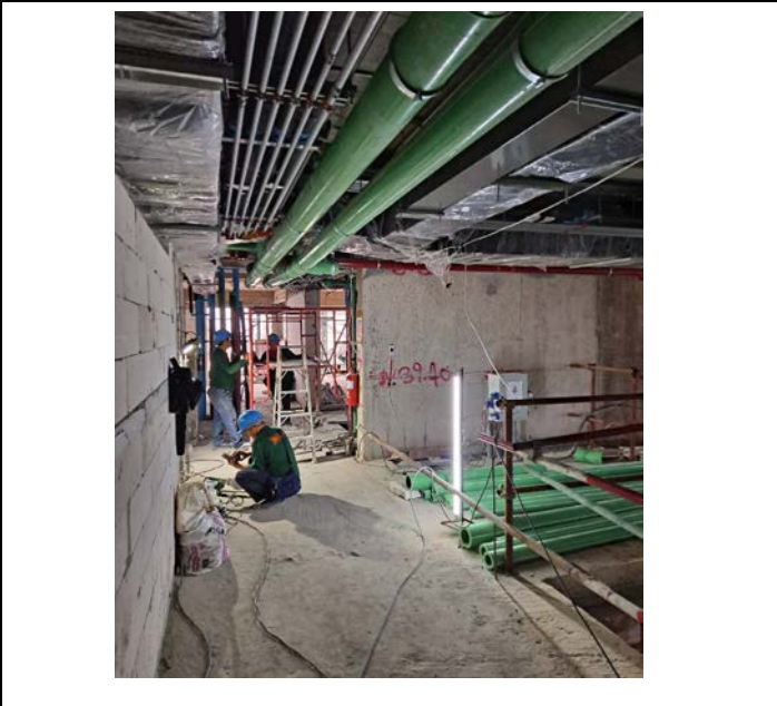
Activity Installation CW,HW Pipe Area Corridor. Floor 12 Date : 18 September 2563
