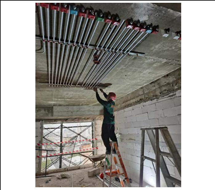
Activity Installation of Electrical Pipe Above the ceiling for the Room. Floor 13 Date : 18 September 2563
