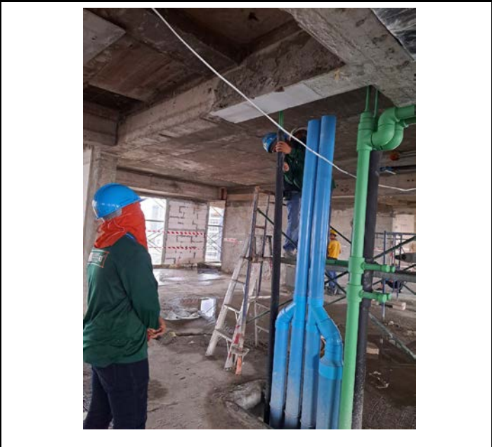
Activity Installation CW,HW Pipe Area Shaft Raiser Floor 16 Date : 18 September 2563
