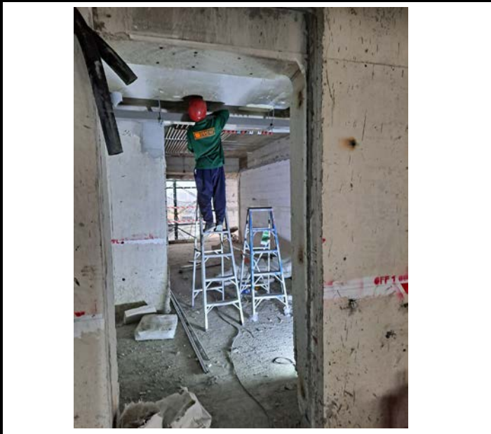
Activity Installation of Electrical Pipe Above the ceiling for the Room. Floor 13 Date : 19 September 2563
