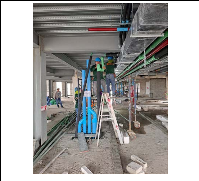
Activity Installation CW,HW Pipe For The Main Shaft. Floor 16 Date : 19 September 2563
