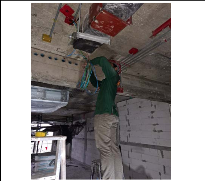
Activity Electrical Wiring Work For The Room. Floor 08 Date : 19 September 2563
