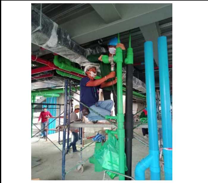
Activity Installation CW,HW Pipe For The Main Shaft. Floor 16 Date : 20 September 2563
