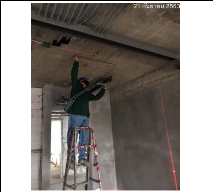
Activity Installation of Air Conditioner Floor 09 Date : 21 September 2563
