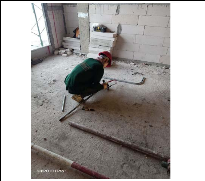
Activity Installation of Electrical Pipe Above the ceiling for the Room. Floor 11 Date : 22 September 2563
