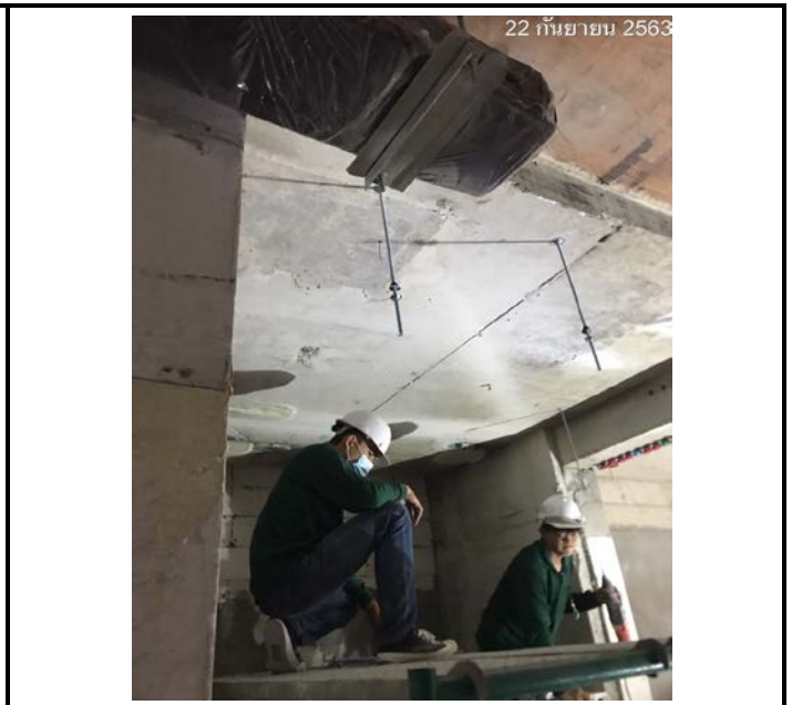
Activity Installation of Air Conditioner Floor 09 Date : 22 September 2563
