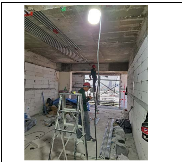
Activity Installation of Electrical Pipe Above the ceiling for the Room. Floor 14 Date : 22 September 2563
