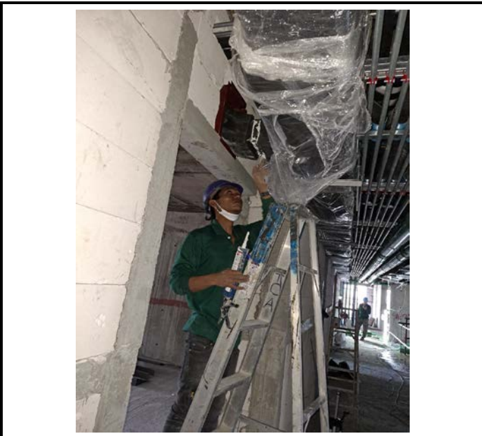
Activity Installation of Duct In The Room Floor 12 Date : 22 September 2563
