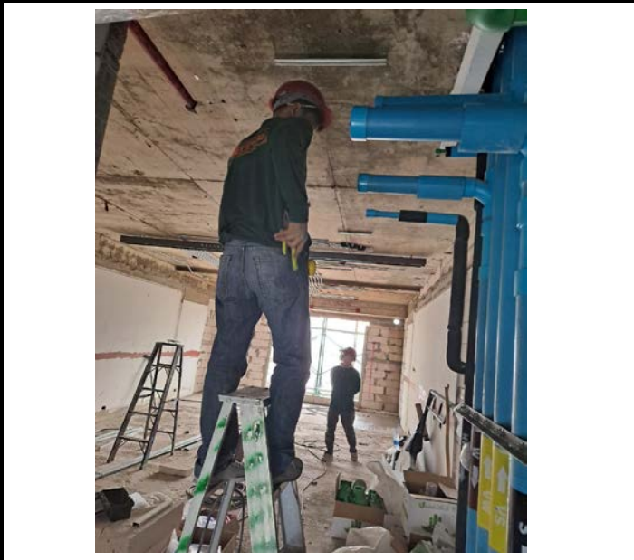
Activity Installation of Electrical Pipe Above the ceiling for the Room. Floor 12 Date : 24 September 2563
