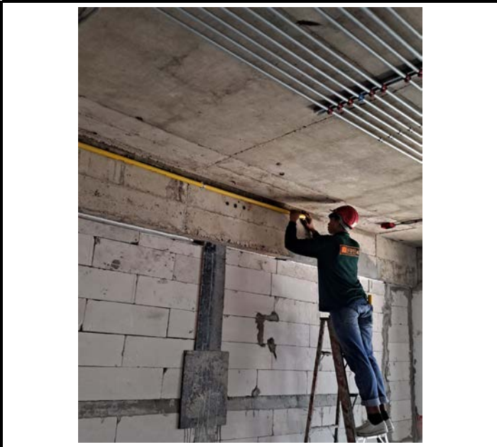
Activity Installation of Grounding System Pipe Floor 08 Date : 24 September 2563
