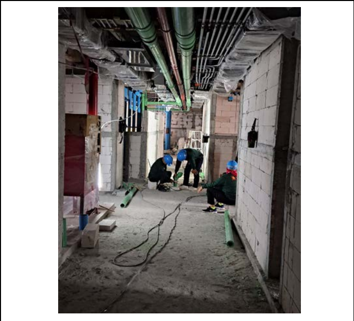
Activity Installation CW,HW Pipe For Corridor Floor 12 Date : 24 September 2563
