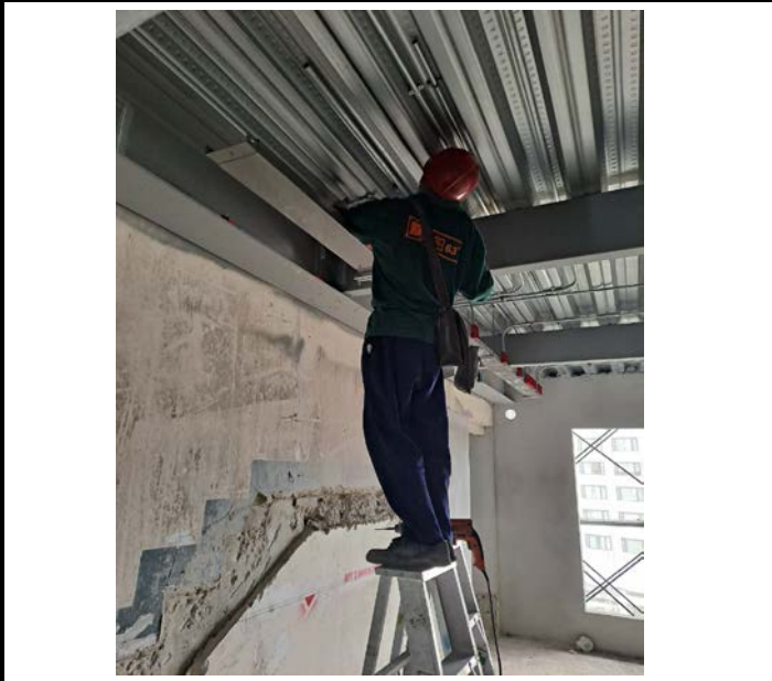
Activity Installation of Electrical Pipe Above the ceiling for the Room. Floor 10 Date : 24 September 2563
