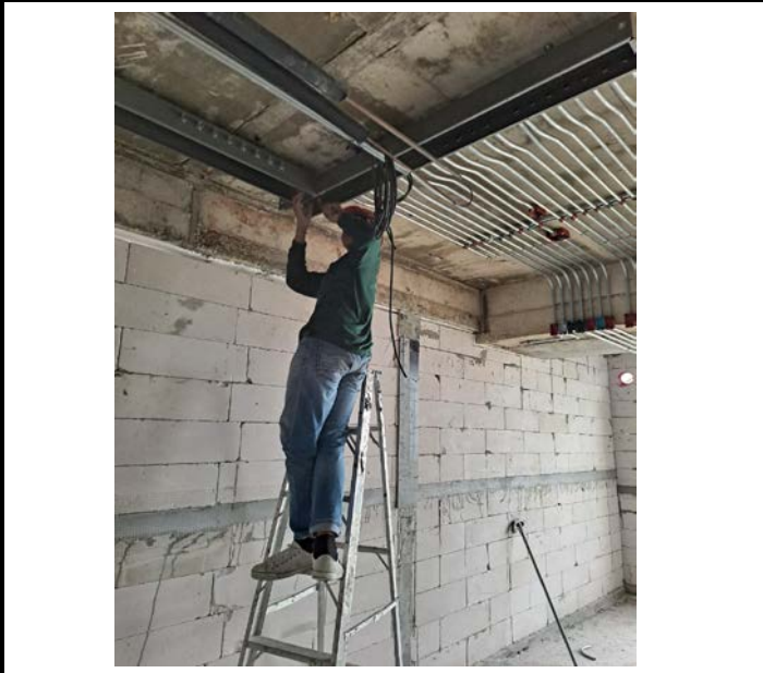
Activity Installation of Electrical Pipe Above the ceiling for the Room. Floor 12 Date : 26 September 2563
