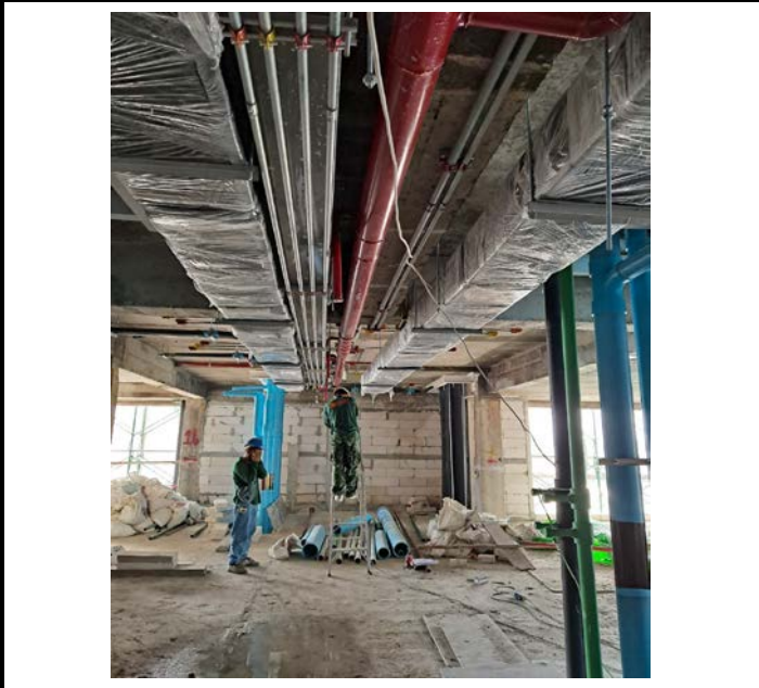
Activity Installation of the Exhaust Fan Duct Floor 08 Date : 26 September 2563
