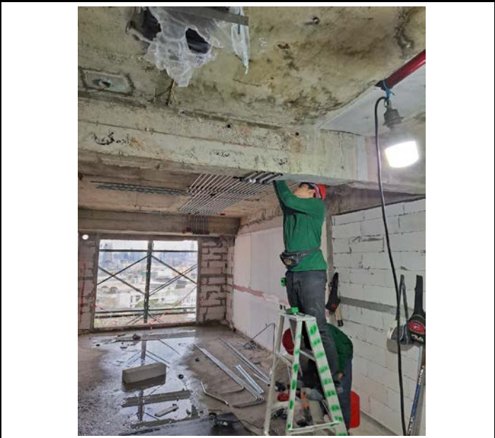
Activity Installation of Electrical Pipe Above the ceiling for the Room. Floor 12 Date : 29 September 2563
