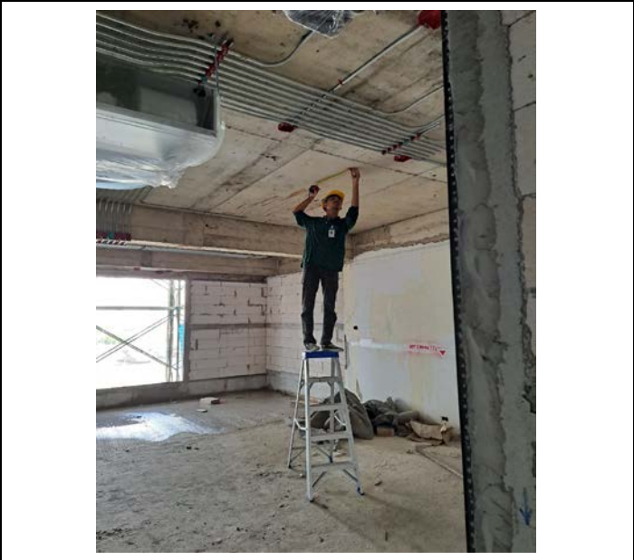
Activity Installation of Electrical Pipe Above the ceiling for the Room. Floor 11 Date : 29 September 2563
