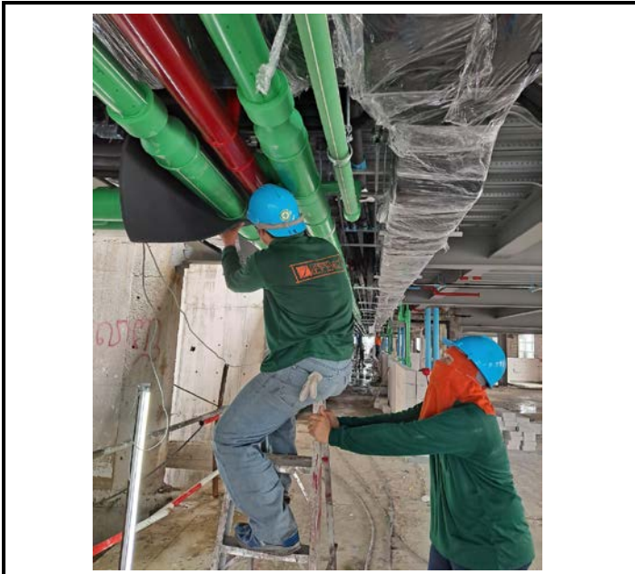
Activity Insulated Cold And Hot Water Pipes At the Corridor Floor 16 Date : 29 September 2563
