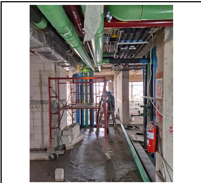
Activity Installation CW,HW Pipe For Shaft Floor 12 Date : 29 September 2563
