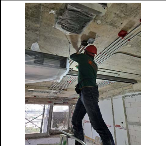
Activity Installation of Electrical Pipe Above the ceiling for the Room. Floor 11 Date : 30 September 2563
